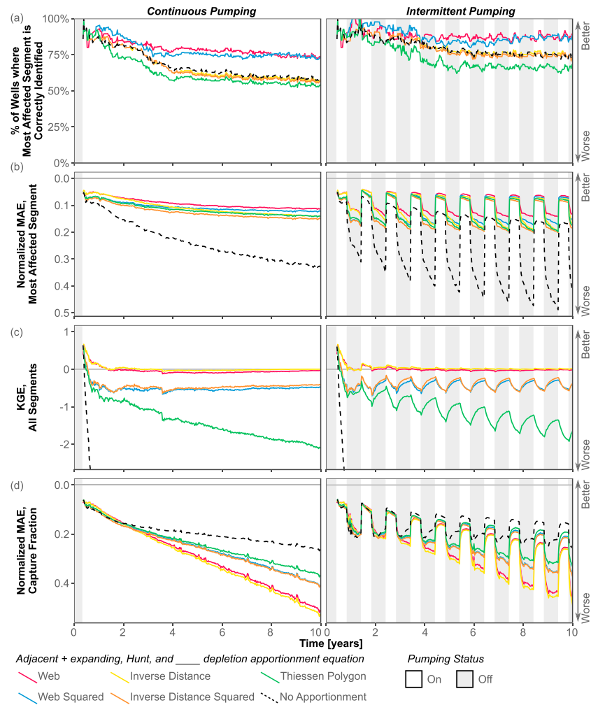
Figure 5. Comparison across depletion apportionment equations for each performance metric. (a) Spatial distribution of primary impact for segments with depletion potential > 5%, (b) magnitude of primary impact, and (c) spatial distribution of overall impacts; (d) magnitude of overall impacts. The “No Apportionment” line shows the performance of the Hunt analytical model without considering stream proximity criteria or depletion apportionment equations. Left column shows continuous pumping experiment and right column is intermittent pumping experiment. Results shown are for Hunt analytical model and adjacent + expanding stream proximity criteria compared to MODFLOW model using RIV for stream features.
