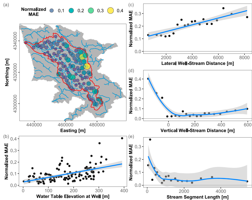
Figure 9. Normalized mean absolute error (MAE) during the final year of the continuous pumping experiment for each well, shown by (a) position within domain, with the MODFLOW domain colored gray and streams colored blue; (b) steady state water table elevation; (c) lateral distance between the well and stream segment; (d) vertical distance between well and stream segment, where a negative value means the well is at a lower elevation than the stream; and (e) stream segment length. For each plot, the variable on the x axis was divided into 20 quantiles used to calculate normalized MAE. The blue lines in (b) and (c) are linear best fit ( R^2 = 0.29 and R^2 = 0.72 , respectively; p < 10^{-5} for both), and the blue lines in (d) and (e) are smoothed loess filters. MODFLOW model with RIV stream features used for evaluation; see Figure S12 for comparison with MODFLOW SFR model.
