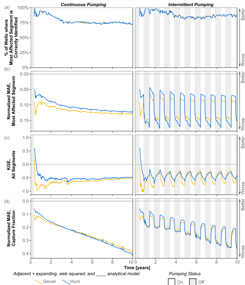
Figure 6. Comparison across analytical models for each performance metric. (a) Spatial distribution of primary impact, (b) magnitude of primary impact, (c) spatial distribution of overall impacts, and (d) magnitude of overall impacts. Note that y axis is reversed on (b) and (d) so that upwards indicates better performance. Left column shows continuous pumping experiment and right column is intermittent pumping experiment. Results shown are for adjacent + expanding stream proximity criteria and web squared depletion apportionment equation compared to MODFLOW model using RIV for stream features.
