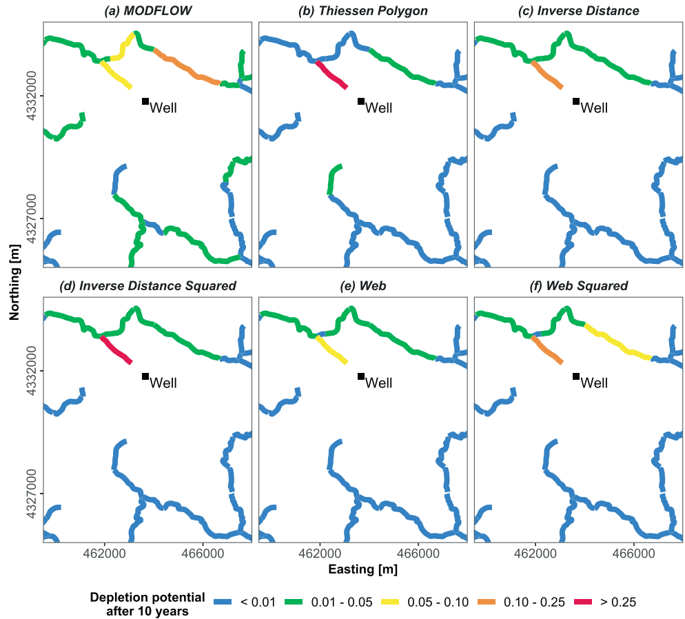
Figure 3. Example of the predicted distribution of depletion among stream segments from a well after 10 years of pumping from (a) MODFLOW and (b-f) each of the depletion apportionment equations, combined with the Hunt analytical model and adjacent + expanding stream proximity criteria. The time series of depletion associated with this well is shown in Figure S7 (“Near” well).
