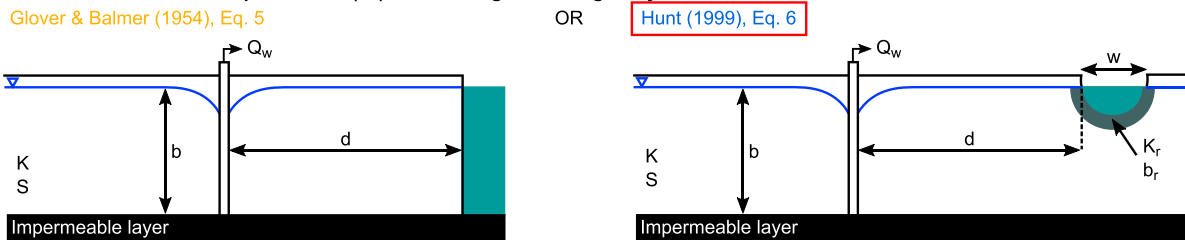
Figure 1. Diagram showing components of an analytical depletion function for a sample stream network. For each step, the option boxed in red is the option with the best overall performance (section 4.2). Colors in component labels correspond to color-coding in Results plots.
