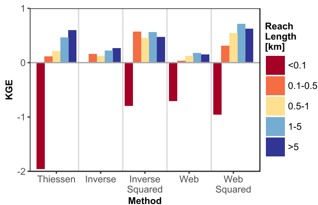
Figure 5. Performance of each depletion apportionment relative to MODFLOW as a function of stream reach length. See supporting information Figure S2 for distribution of stream reach lengths in each domain.
