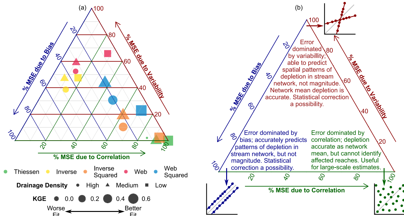
Figure 6. Ternary diagrams visualizing overall fit (KGE) and contribution of bias, variability, and correlation to total error (MSE). (a) Comparison between depletion apportionment equations and drainage density for flat, no recharge simulations. Shapes are size-coded by KGE, such that larger points have a better overall fit. (b) Annotated ternary diagram highlighting relevance of different types of error to streamflow depletion management. Pop-out scatterplots show examples analogous to Figure 4 for each endmember point of the ternary diagram.
