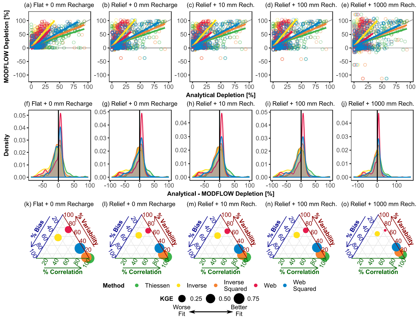
Figure 7. Sensitivity to topographic relief (“Flat” or “Relief” in plot labels) and recharge (rate in plot labels) for low density domain. (a), (f), and (k) are the same as Figures 4c and 4f, and low density points in Figure 6a, respectively.
