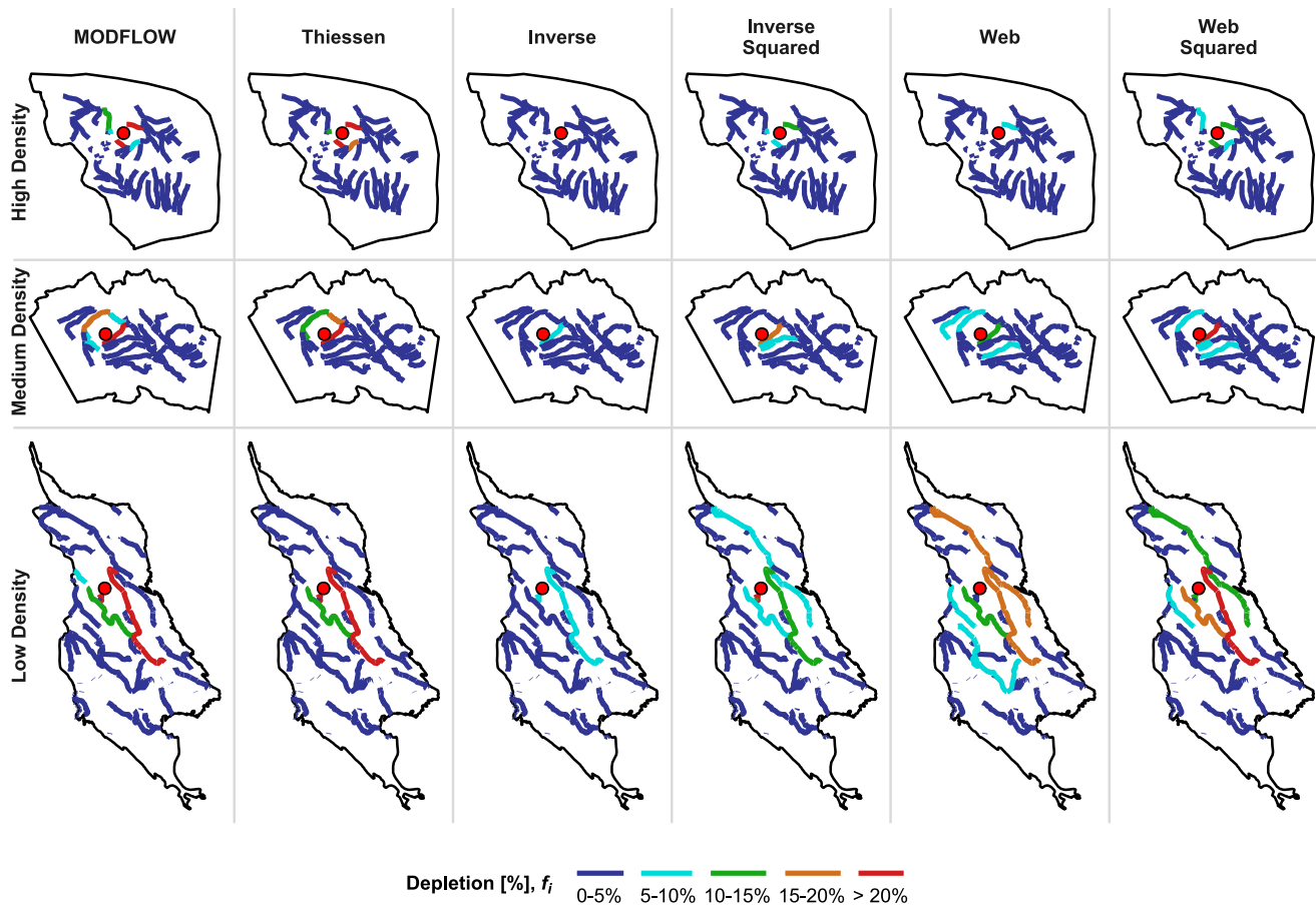
Figure 3. Example plot showing estimated depletion for different stream reaches under each apportionment method for a single pumping well (red dot). Supporting information Figure S1 shows a map of depletion for a given reach.
