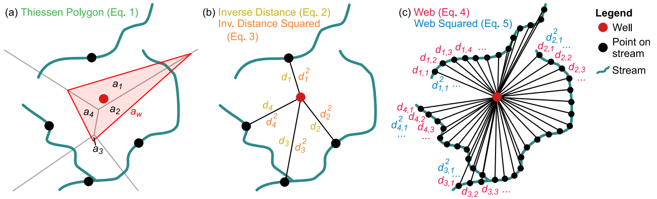
Figure 2. Diagrams showing (a) Thiessen polygon, (b) inverse distance, and (c) web inverse distance apportionment methods. Black dots in Figures 2a and 2b are the points on the stream closest to the well. Letters correspond to variables in equations (1)–(5).
