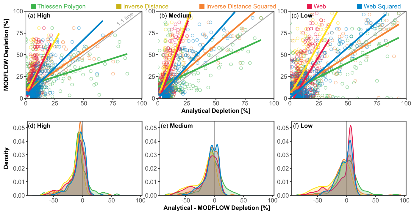
Figure 4. Performance of each method and domain; only well/reach combinations with a depletion of >5\% included. (a–c) MODFLOW versus analytical depletion apportionment for high, medium, and low drainage density domains. All linear best-fit lines are statistically significant ( p < 0.05 ). (d–f) Difference between analytical and MODFLOW approaches for high, medium, and low drainage density domains.
