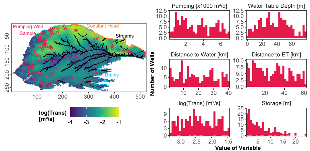
Figure 2. (Left) Map showing Republican River Compact Administration MODFLOW model domain, hydrostratigraphic properties, and selected pumping wells for pumping experiment. \log(\text{Trans}) is log-10 transformed transmissivity. (Right) Properties of wells sampled for pumping experiment, which are described in detail in Section 2.3.1 of the text.
