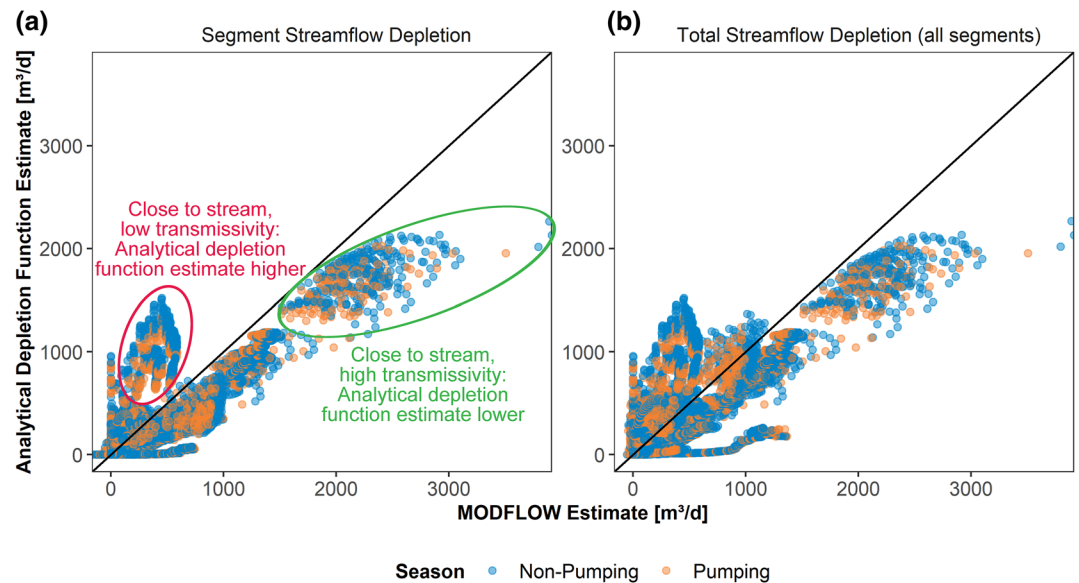
Figure 3. Comparison between analytical depletion function and MODFLOW predictions of (a) segment-scale streamflow depletion, (b) total streamflow depletion summed across all segments for a given well. Circles on depletion plot indicate “higher estimate” and “lower estimate” points discussed in Section 3.1 text.
