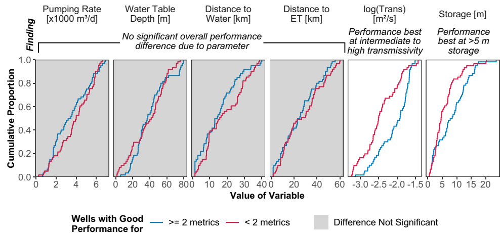
Figure 5. Regional sensitivity analysis results, expressed as empirical cumulative distribution functions for wells with good performance in at least two fit metrics and wells with good performance in less than two fit metrics. In shaded panels, distributions of the two samples are expected to be drawn from the same distribution (two-sample Kolmogorov-Smirnov test p > 0.05 ).
