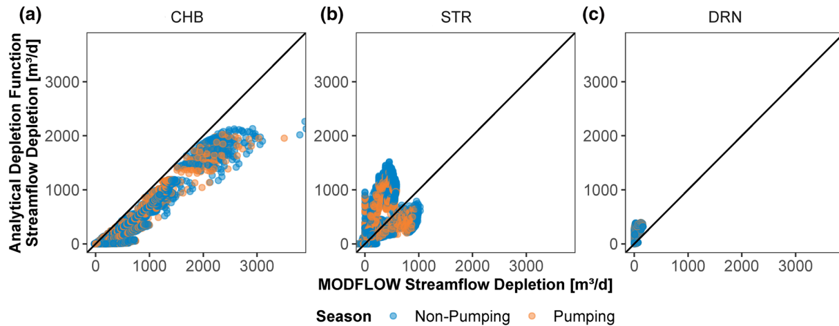
Figure 4. Comparison between analytical depletion function and MODFLOW predictions of segment-scale streamflow depletion for (a) CHB package, (b) STR, and (c) DRN in MODFLOW. CHB, constant head boundary; DRN, drain package; STR, stream package.
