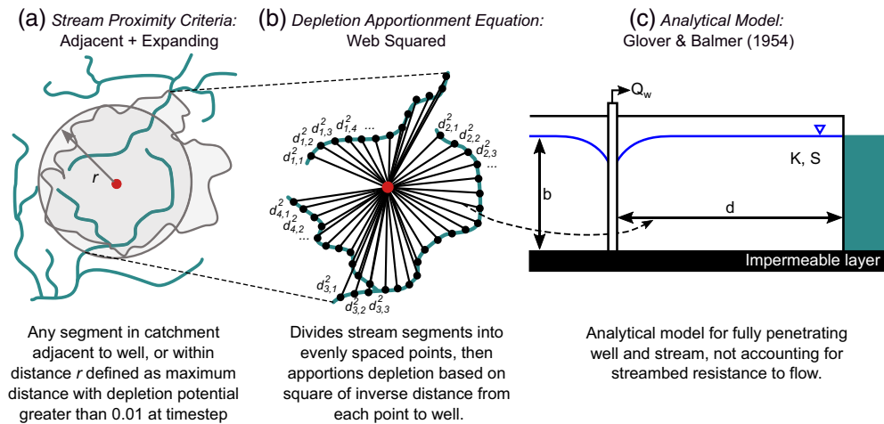
Figure 1. Components of an analytical depletion function: (a) stream proximity criteria, which identify stream segments that may be affected by a well; (b) a depletion apportionment equation, which divides streamflow depletion caused by the well among affected segments; (c) an analytical model, which calculates the depletion in each individual stream segment. Modified from Zipper, Carah, et al. (2019) under CC-BY 3.0 license.
