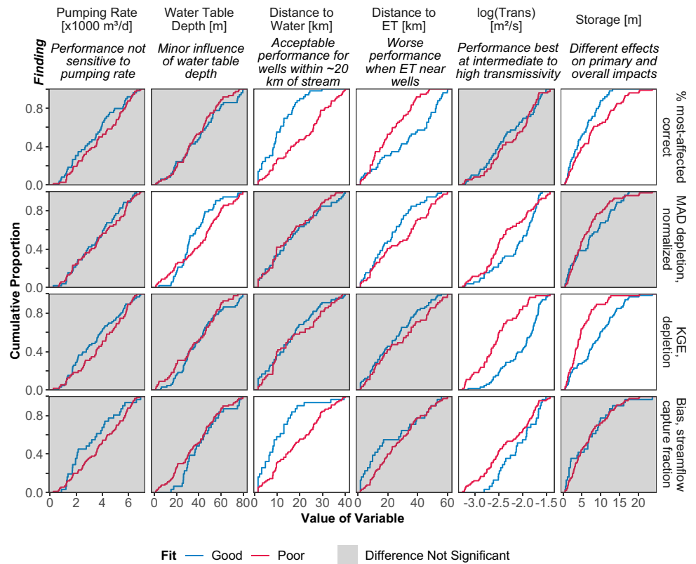
Figure 6. Regional sensitivity analysis results, expressed as empirical cumulative distribution functions for well characteristics for each performance criteria. In shaded panels, distributions of “good” and “poor” groups are expected to be drawn from the same distribution (two-sample Kolmogorov-Smirnov test p > 0.05 ).
